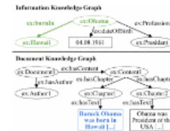
Information-KG and Document-KG.
